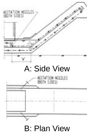
Fig 30: Matimba SSC - location of agitation nozzles
