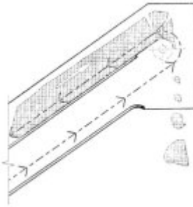
Fig.3: Ash load on dewatering slope during "Backlog Recovery"
