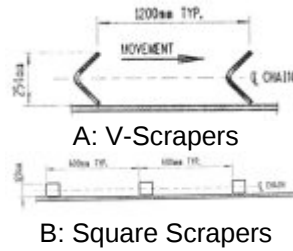
Fig 4: Types of Scrapers Tested
