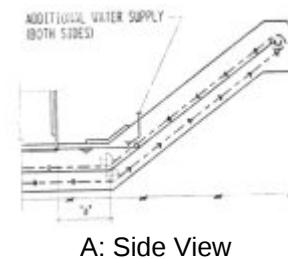
Fig 31: Geometry of intersection areas of Matimba/Kendal SSCs
